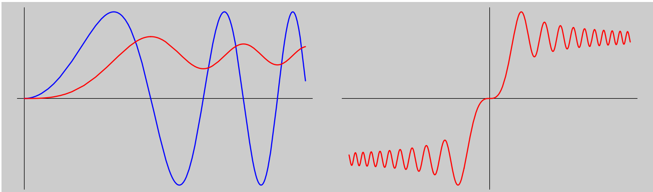
Fig. The Fresnel function S(x) = \int_0^x \sin(\pi t^2/2) dt .
