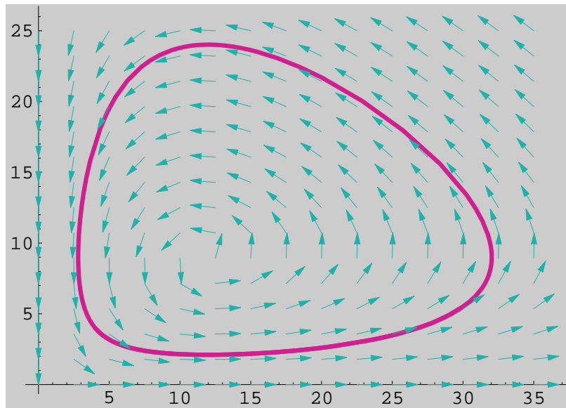
Fig. Cyclic predator-prey system
